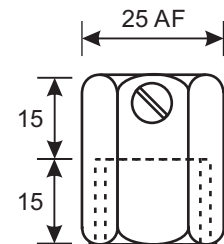
1/2" BSP Female
