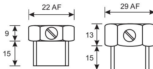
1/2" BSP Male
